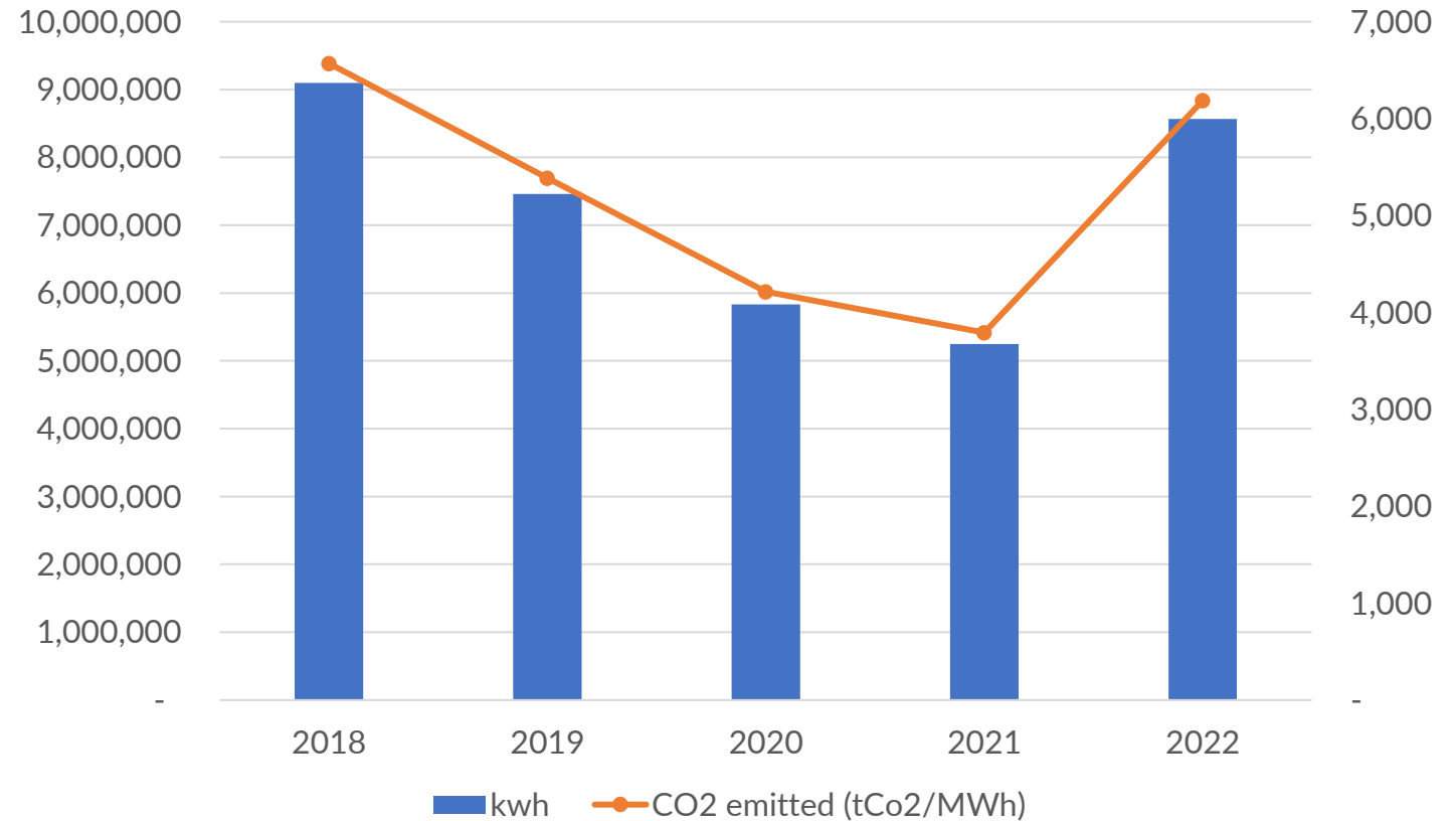
Scope 1 emissions 2018-2022
